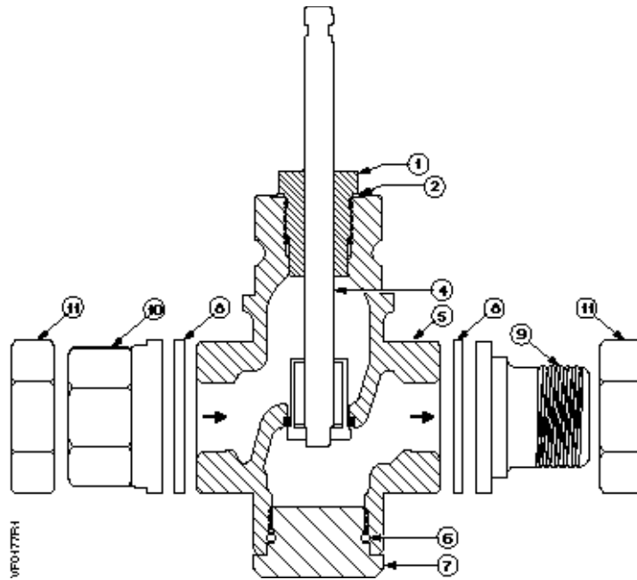
Figure 7. Normally Closed 1/2-inch to 2-inch (15 to 50 mm) Line Size Valve.
