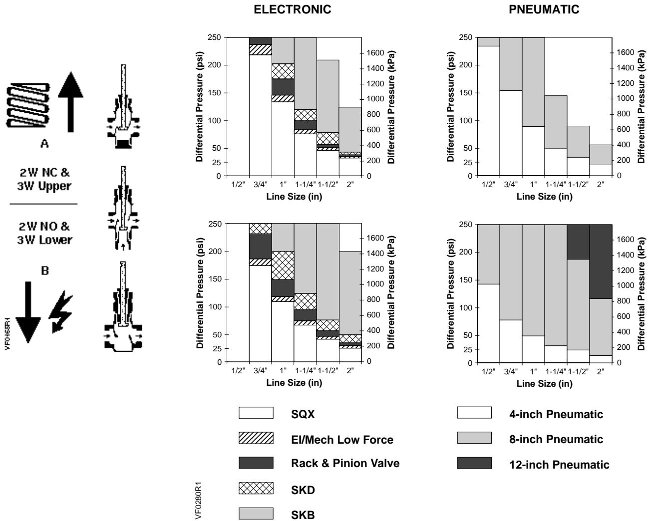
Figure 4. Close-off Pressures.
