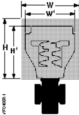
Figure 6. Dimensions.
