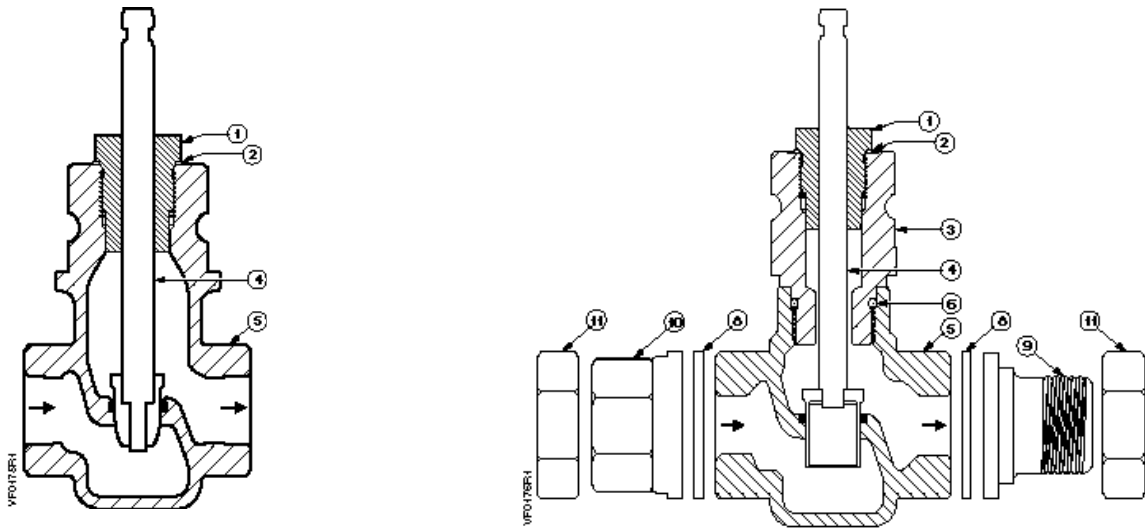
3/4-inch to 2-inch (20 to 50 mm) Line Size Valve
